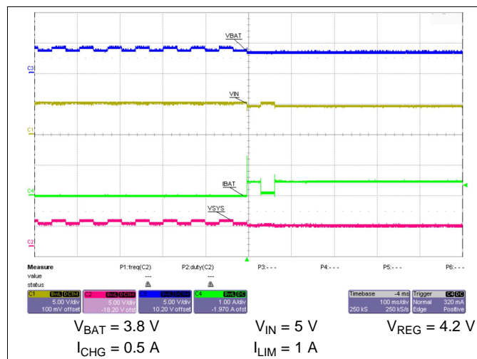
Figure 1. Battery Detection
