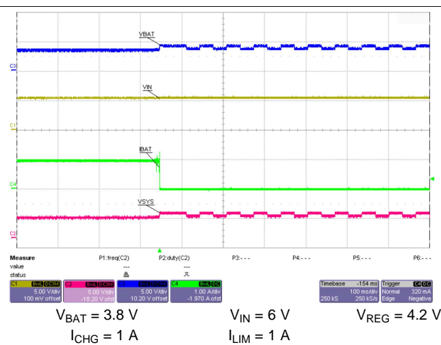
Figure 2. Battery Removal
