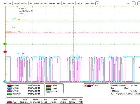
Figure 32. I²C READ (Address=31d, Cmd=0x79): ACK 0x10C8. Ioc = 15 A
