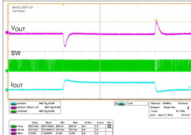
Figure 59. Load Transient
