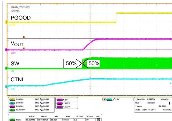
Figure 57. Start-Up Sequence
