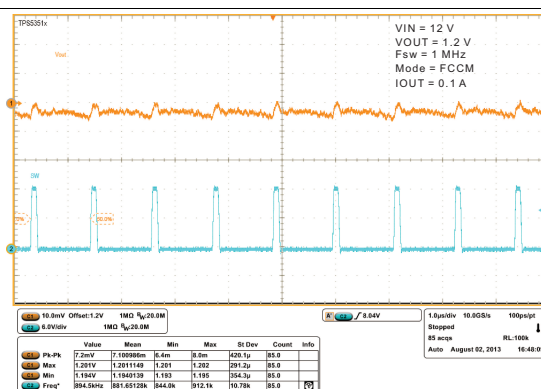
Figure 16. FCCM Steady-State Operation
