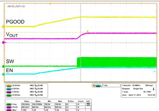
Figure 64. Pre-Bias Start-Up
