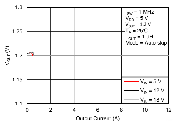
Figure 54. Output Voltage vs. Output Current
