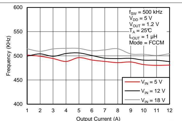
Figure 56. Switching Frequency vs. Output Current
