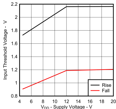
Figure 7-16. Input Threshold vs Supply Voltage
