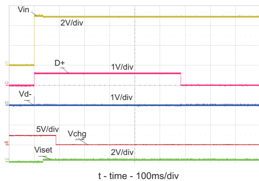
Figure 6-1. D+ D– Detection for Adaptor Hot Plug
