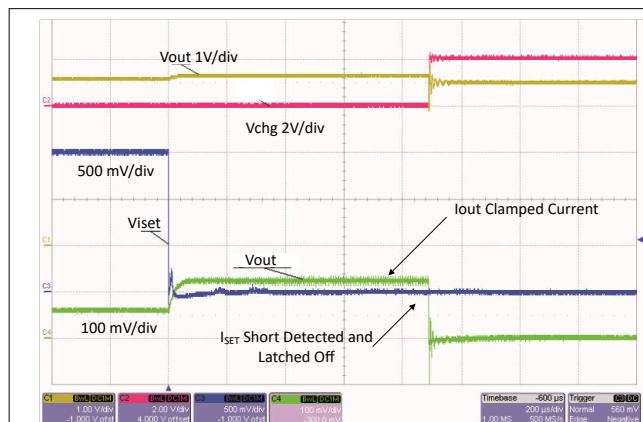
Figure 8-2. ISET Shorted During Normal Operation
