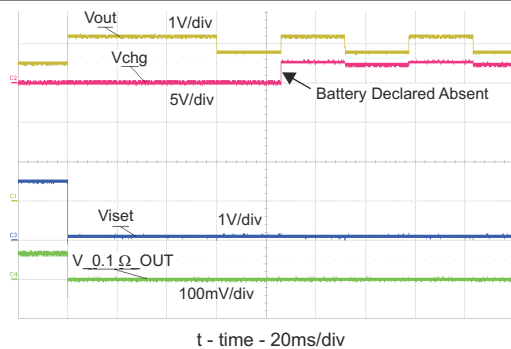
Figure 6-7. Battery Removal With Fixed TS = 0.5 V
