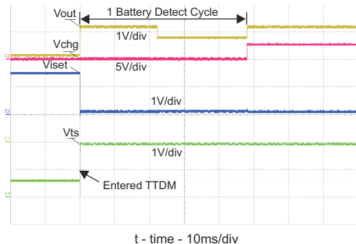
Figure 6-6. Battery Removal With OUT and TS Disconnect First
