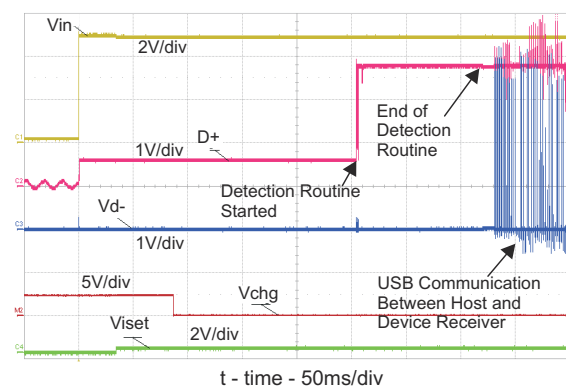
Figure 6-4. D+ D– Detection for USB Hot Plug With Pullup
