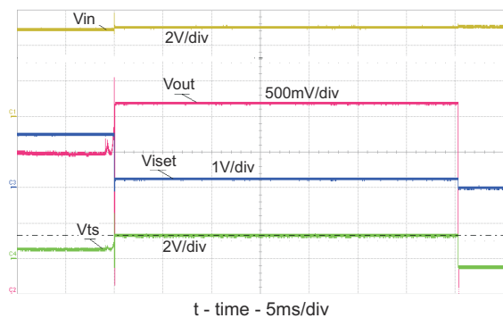
Figure 6-5. Battery Removal – GND Removed First
