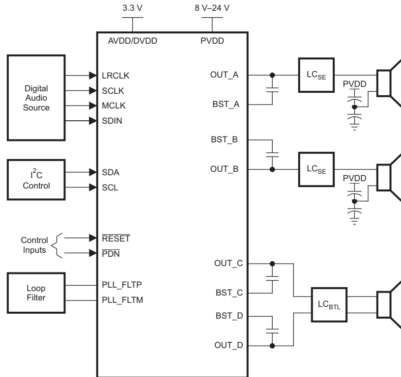
Figure 72. Simplified 2.1 Application Diagram
