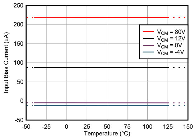
Figure 7-20. Input Bias Current vs Temperature
