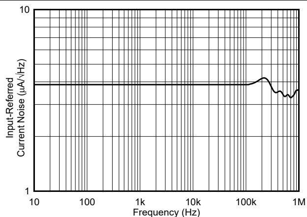
Figure 7-24. INA254A2 Input-Referred Current Noise vs Frequency
