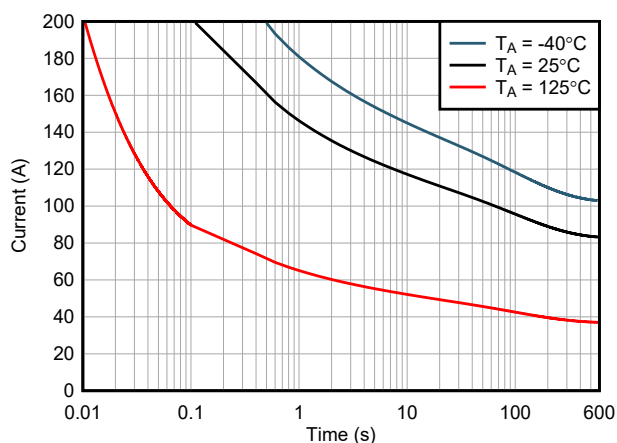
Figure 8-2. Short-Circuit Duration
