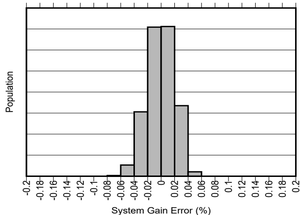
Figure 7-8. Gain Error Production Distribution (INA254A3)
