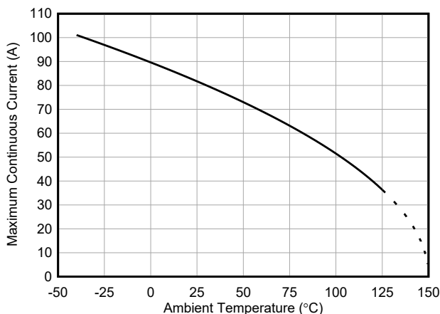
Figure 8-1. Maximum Continuous Current vs Ambient Temperature
