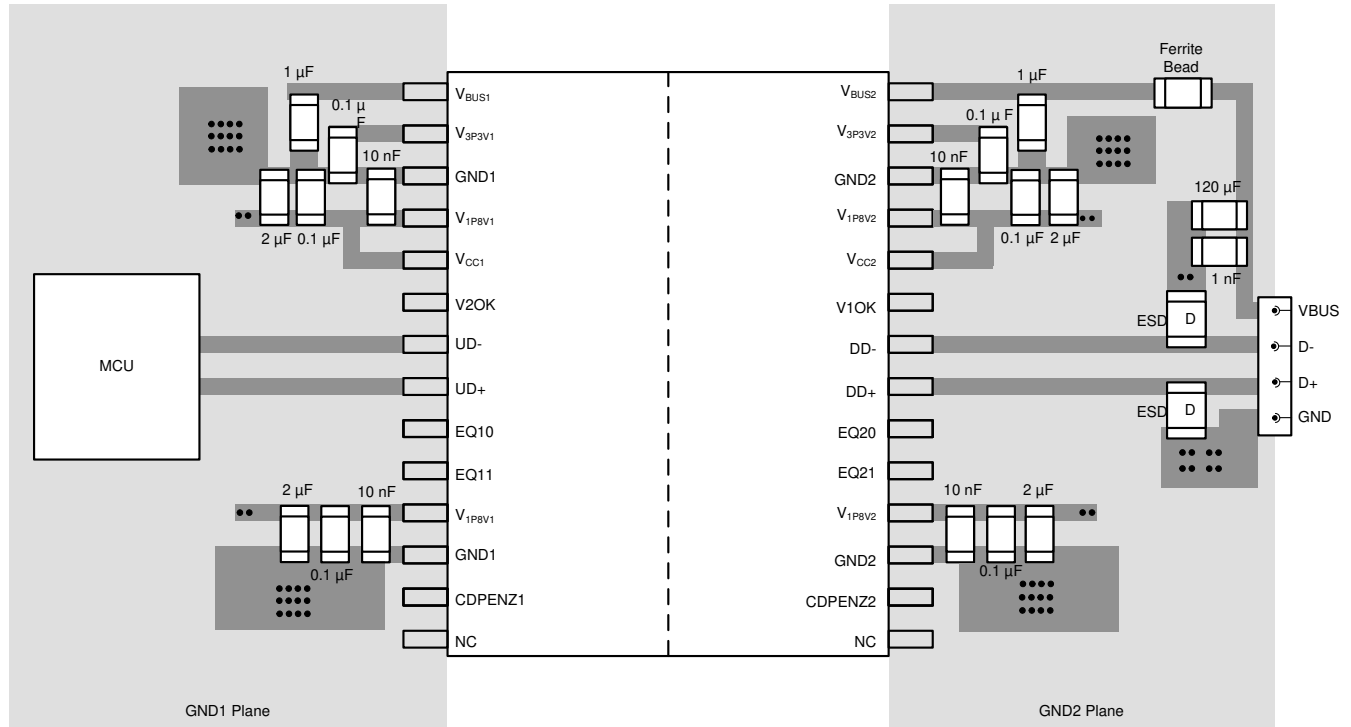
Figure 8-9. Layout Example for ISOUUSB211
