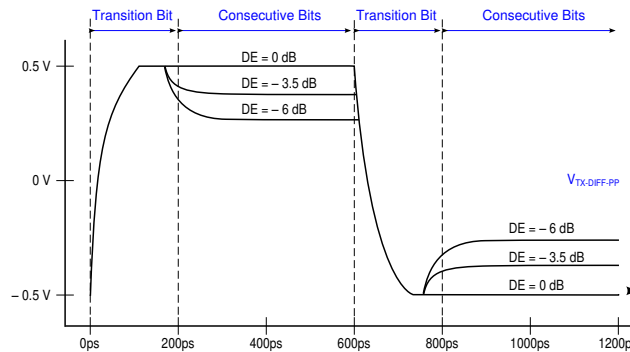
Figure 6-2. Transmitter Differential Voltage in Presence of De-Emphasis
