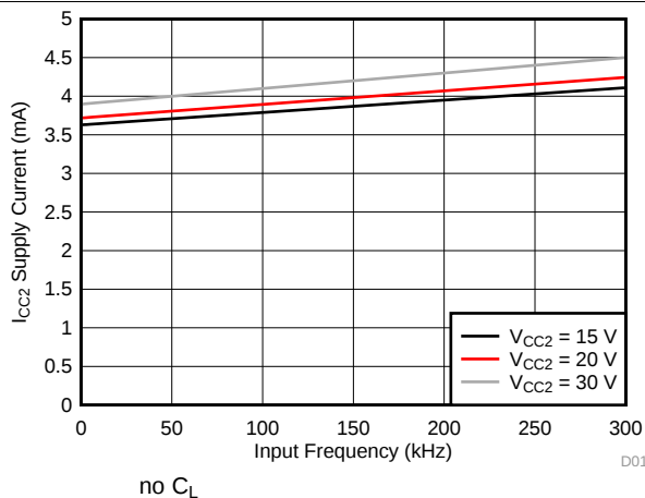
Figure 20. I_{CC2} Supply Current vs Input Frequency
