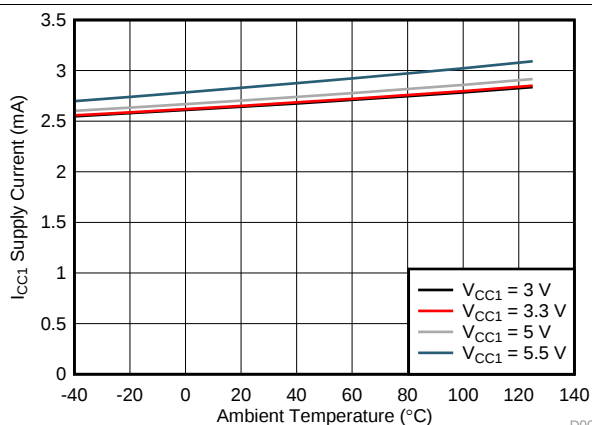
Figure 16. I_{CC1} Supply Current vs Temperature
