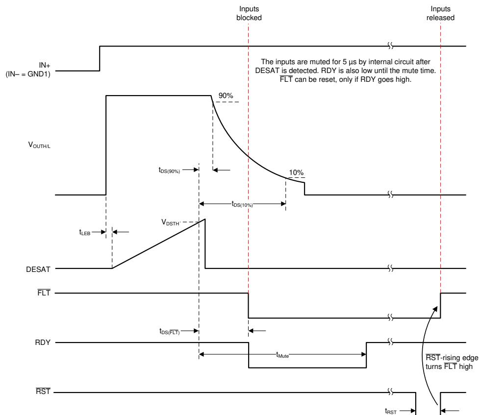
Figure 8-3. DESAT, OUTH/L, \overline{\text{FLT}} , \overline{\text{RST}} Delay
