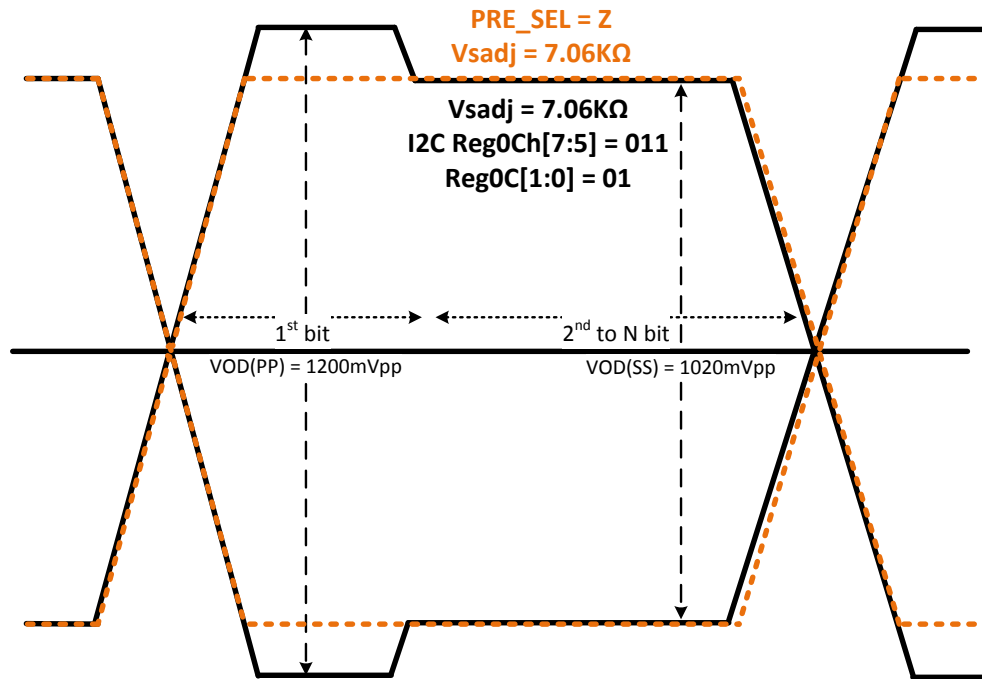
Figure 29. Pre-emphasis Using I²C
