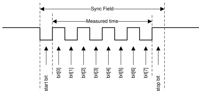
Figure 7-21. UART Sync Field
