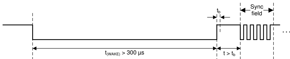
Figure 7-36. UART Wake-Up Pulse
