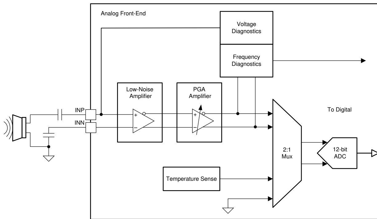
Figure 7-3. Analog Front-End
