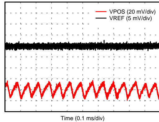
Figure 77. Internal Reference Voltage DC/DC Ripple
