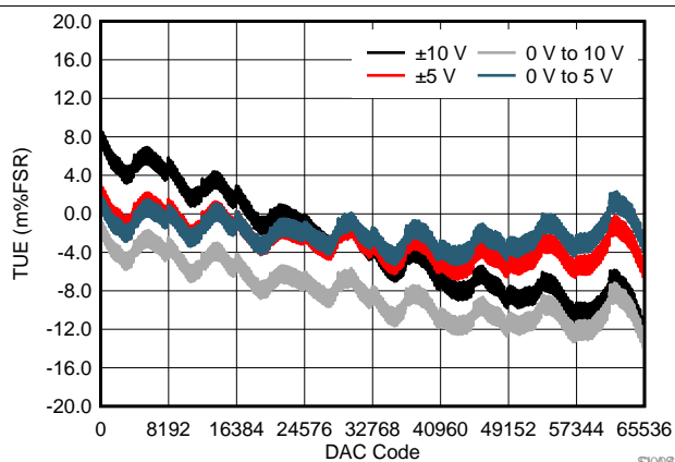
Figure 8. VOUT TUE vs Code (DC/DC Disabled)
