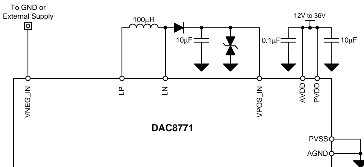
Figure 130. DAC8771 With Single Supply from Internal DC/DC
