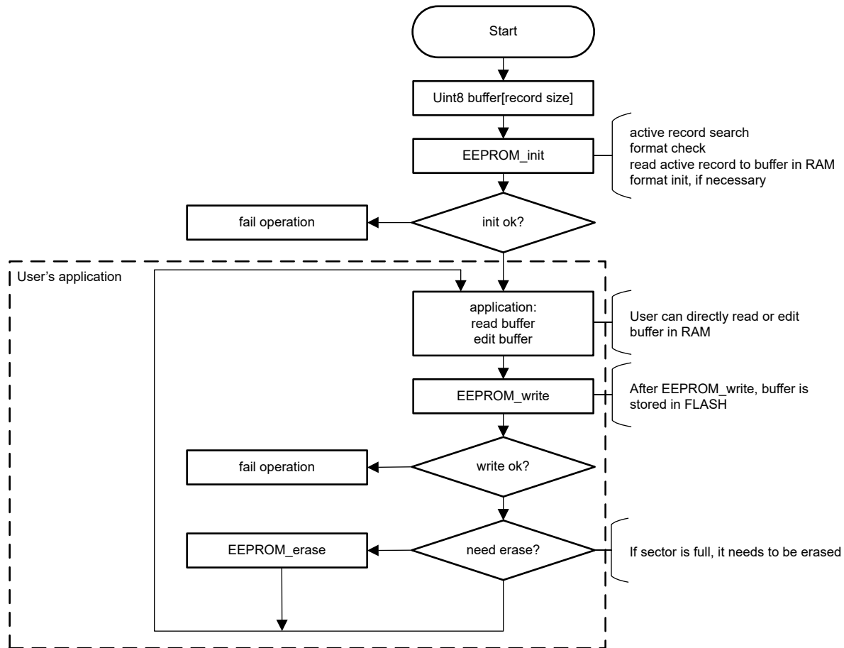
Figure 5-1. Application Software Flow Chart
