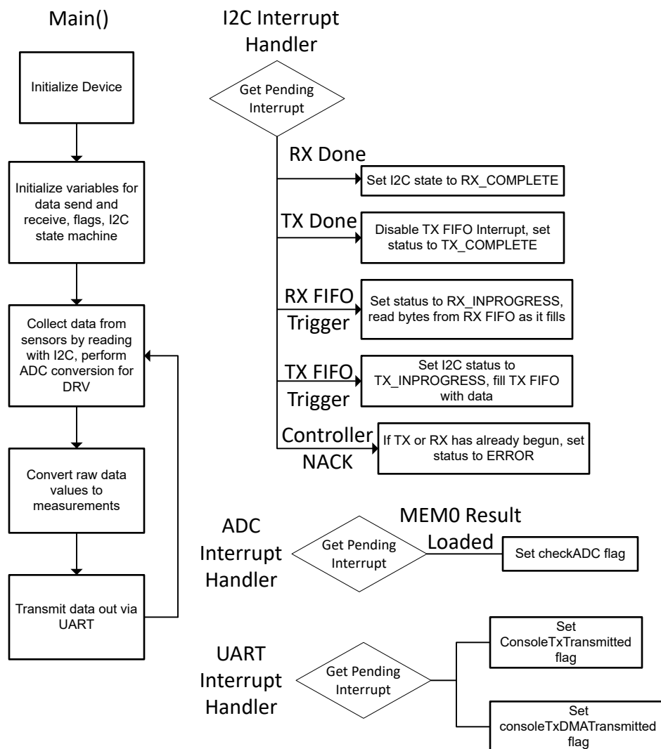
Figure 1-2. Application Software Flowchart
