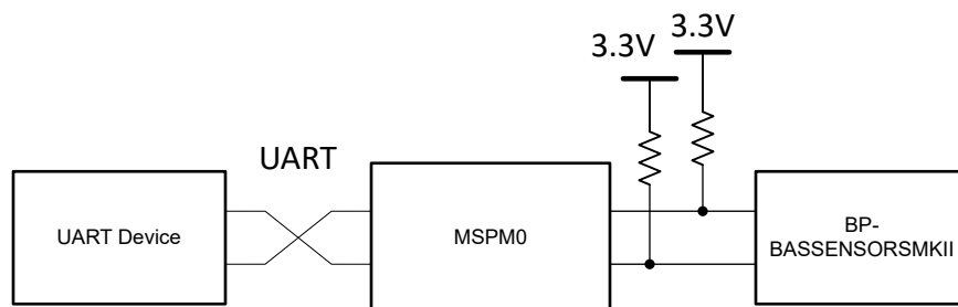
Figure 1-1. System Functional Block Diagram
