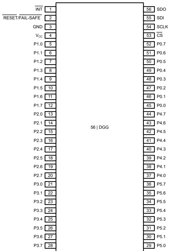
Figure 4-1. Pin Diagram
