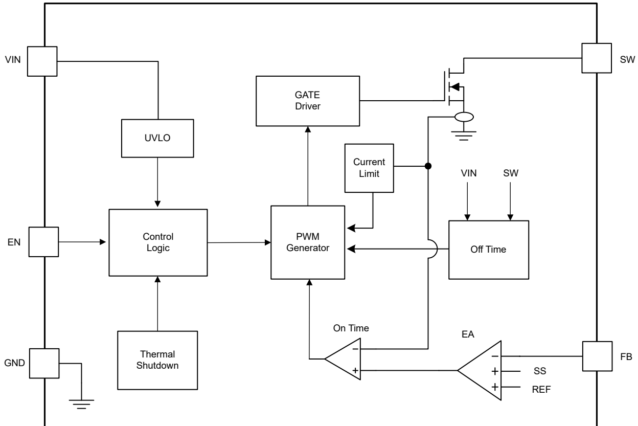
Figure 1-1. TLV61047-Q1 and TLV61040-Q1 Functional Block Diagram
