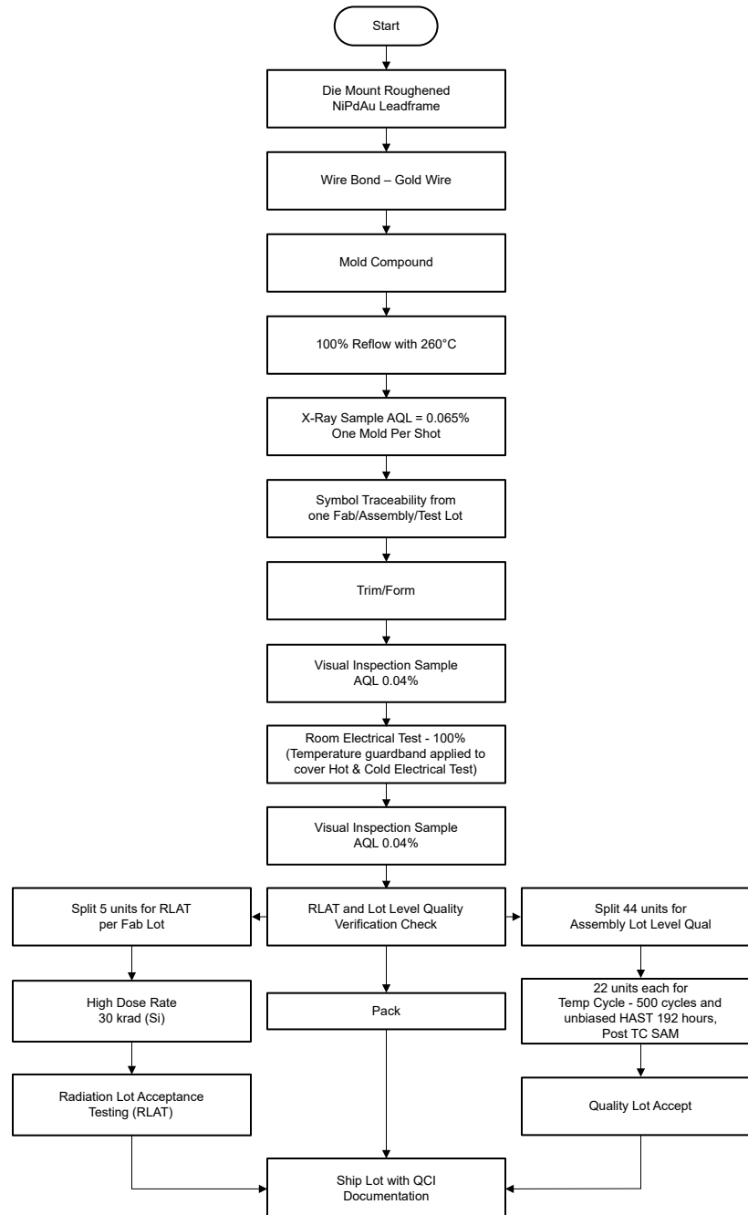
Figure 2-1. SN54SC8T165-SEP Space Enhanced Plastic Production Flow Chart
