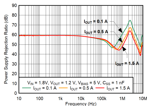
Figure 7-10. V_{\text{BIAS}} PSRR vs Frequency
