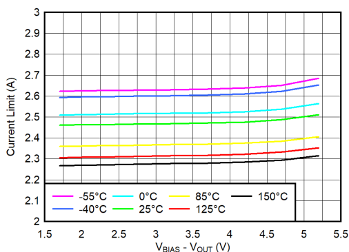
Figure 7-11. Current Limit vs ( V_{\text{BIAS}} - V_{\text{OUT}} )
