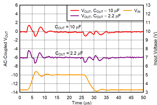
Figure 7-12. V_{\text{BIAS}} Line Transient
