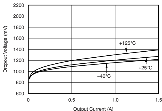
Figure 7-9. V_{\text{BIAS}} Dropout Voltage vs I_{\text{OUT}} and Temperature ( T_J )
