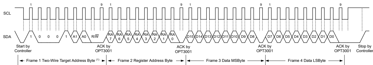
Figure 6-2. I²C Write Example
