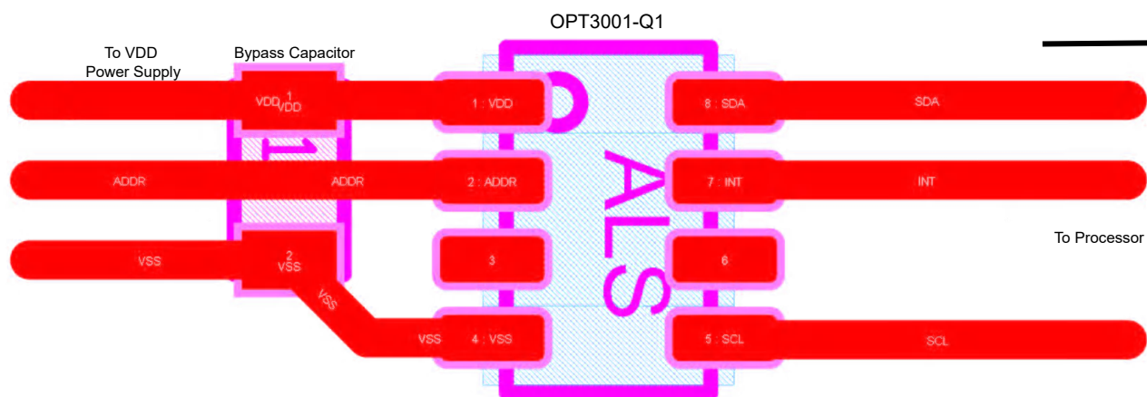
Figure 8-8. OPT3001-Q1 SOT-5X3 Layout Example
