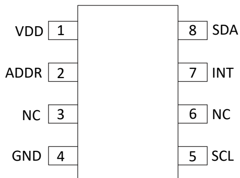
Figure 4-2. DTS Package 8-Pin SOT-5X3 Top View
