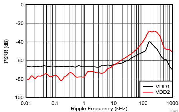
Figure 6-30. Power-Supply Rejection Ratio vs Ripple Frequency
