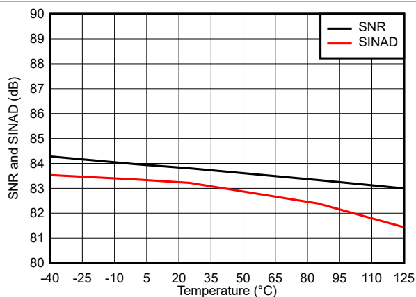
Figure 6-23. Signal-to-Noise Ratio and Signal-to-Noise + Distortion vs Temperature
