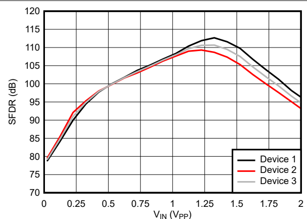
Figure 6-29. Spurious-Free Dynamic Range vs Input Signal Amplitude
