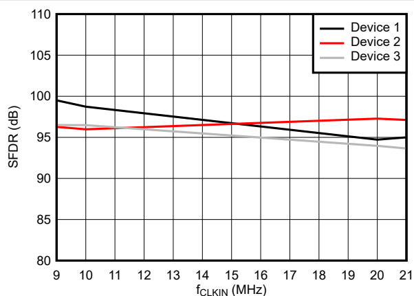
Figure 6-31. Spurious-Free Dynamic Range vs Clock Frequency
