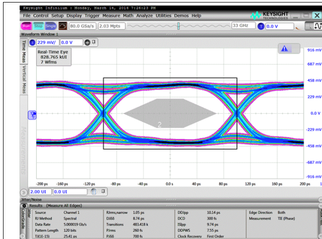
Figure 68. Data Eye at 5 Gbps
