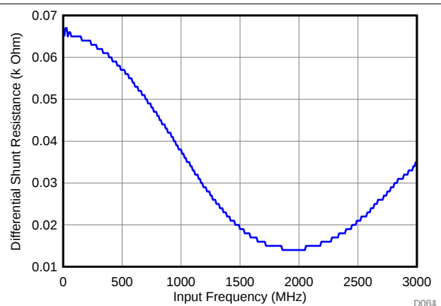
Figure 36. Differential Input Resistance vs Input Frequency
