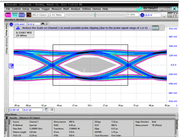
Figure 69. Data Eye at 12 Gbps
