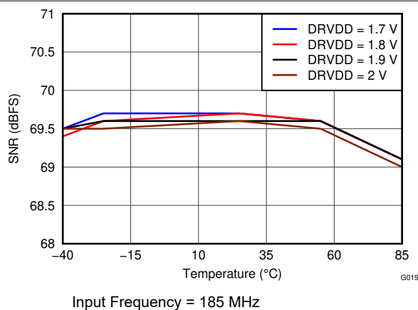
Figure 6-21. Signal-to-Noise Ratio vs DRVDD Supply and Temperature
