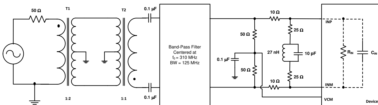
Figure 9-7. Driving Circuit for a 100- \Omega Source Impedance and Input Frequencies in the Third Nyquist Zone
