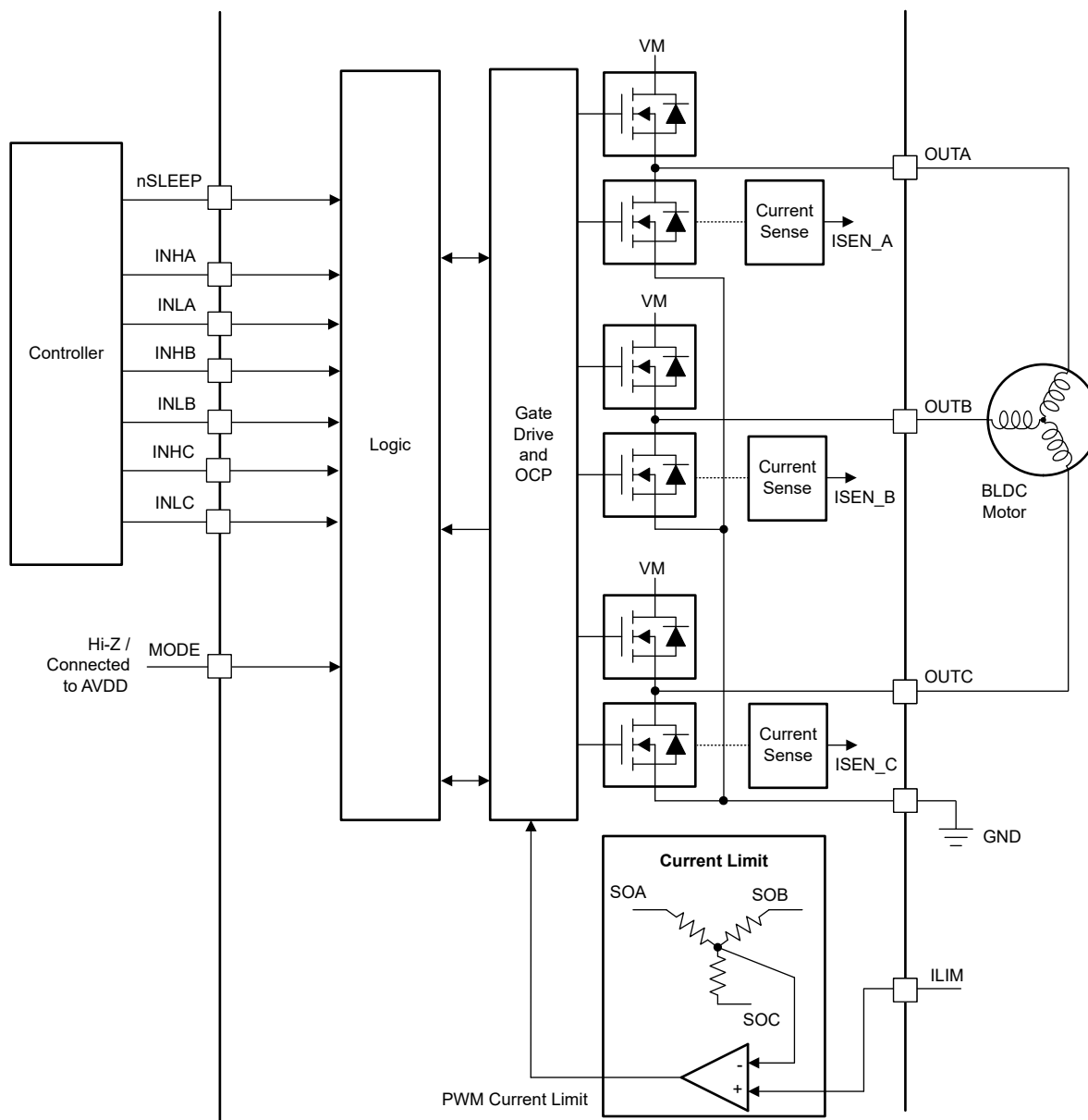
Figure 8-5. Current Limit Mode
