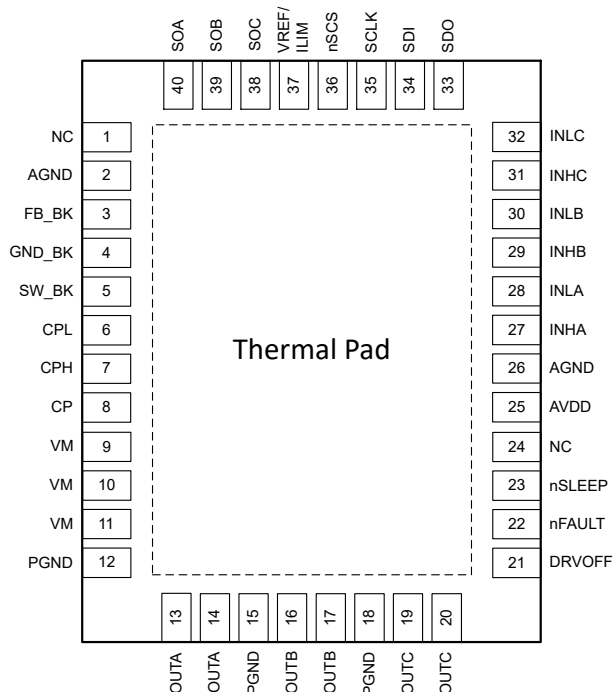
Figure 6-1. DRV8316R 40-Pin VQFN With Exposed Thermal Pad Top View
