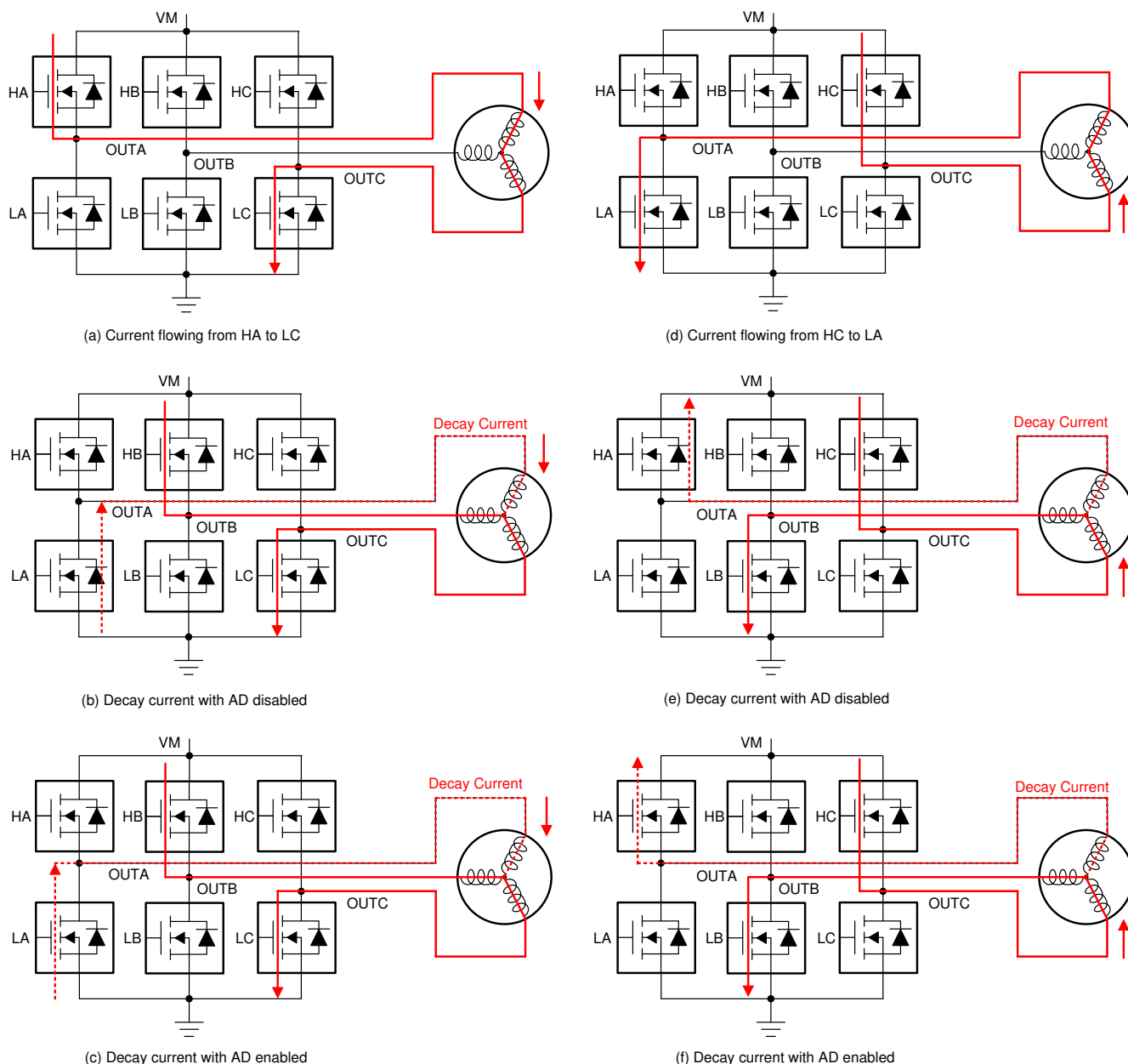
Figure 8-31. ASR in BLDC Motor Commutation
