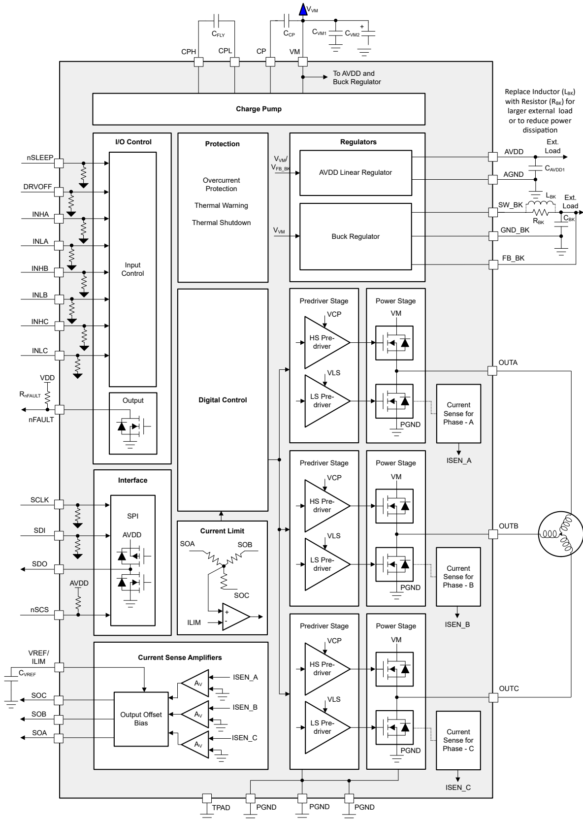
Figure 8-1. DRV8316R Block Diagram
