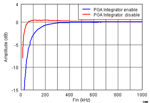
Figure 61. Signal Chain Low Frequency Response with INM Capacitor = 1 \text{ μF}
