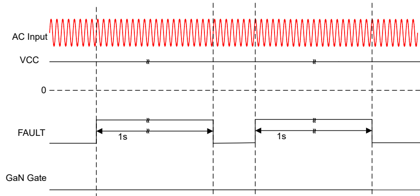
Figure 7-12. Auto-Retry Fault Response
