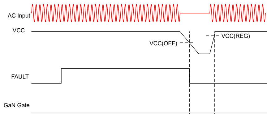
Figure 7-13. Latched Fault Response
