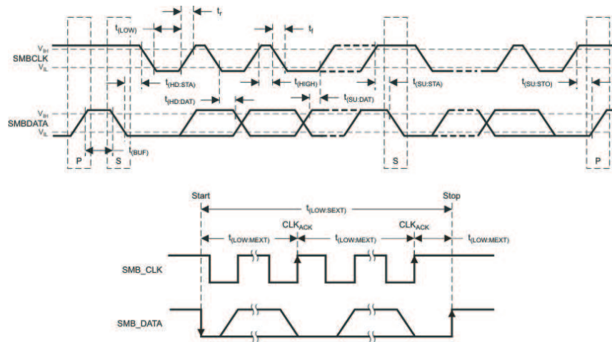
Figure 1. I 2 C/SMBus/PMBus Timing in Extended Mode Diagram
