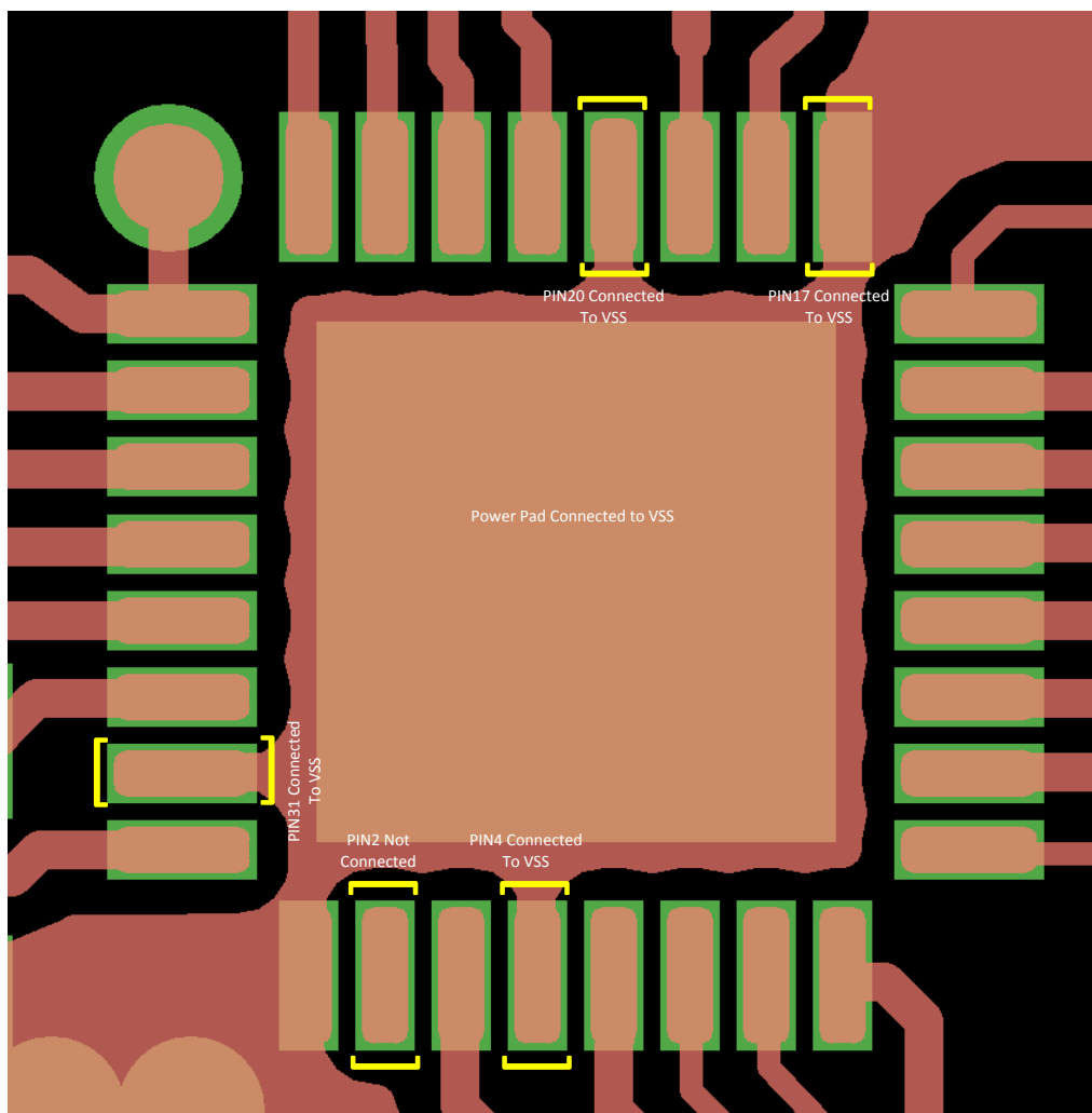
Figure 22. UCD9081 Layout, Top Layer
