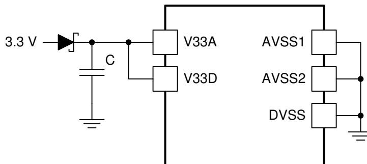
Figure 33. Brownout Circuit
