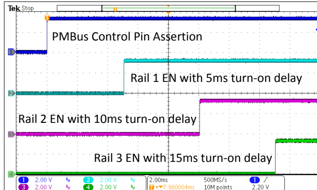
Figure 33. Example Power-on Sequence
