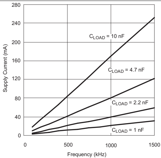
Figure 7. Supply Current vs Frequency ( V_{DD} = 8\text{ V} )
