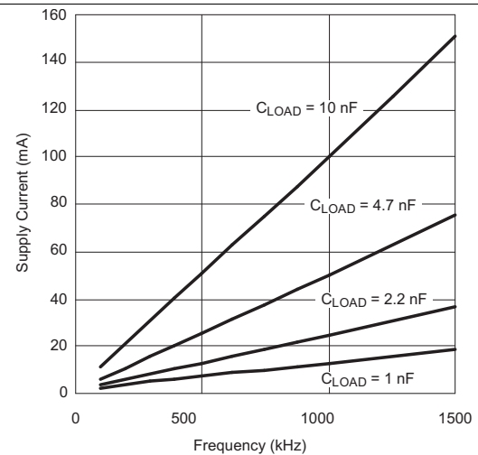
Figure 6. Supply Current vs Frequency ( V_{DD} = 5\text{ V} )
