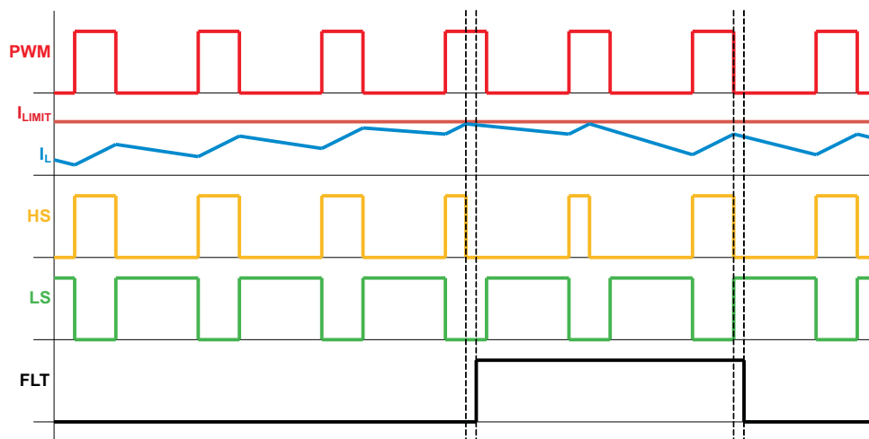
Figure 16. FLT Signal
