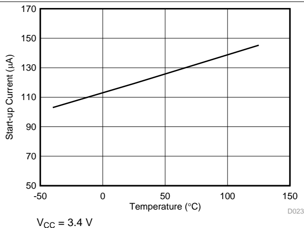
Figure 2. Start-Up Current ( I_{CC(UV)} ) vs Temperature
