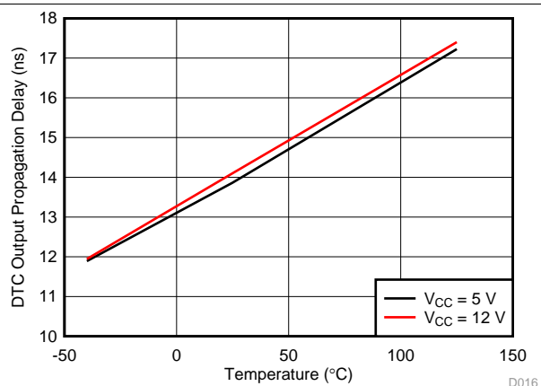
Figure 15. Gate Turnoff Propagation Delay ( t_{d(2)} ) vs Temperature
