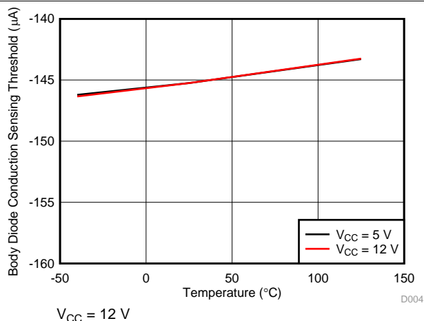
Figure 5. Body-Diode Conduction Sensing Threshold ( V_{TH} ) vs Temperature
