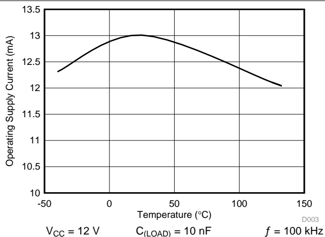
Figure 4. Operating Supply current ( I_{CC(OPERATE)} ) vs Temperature
