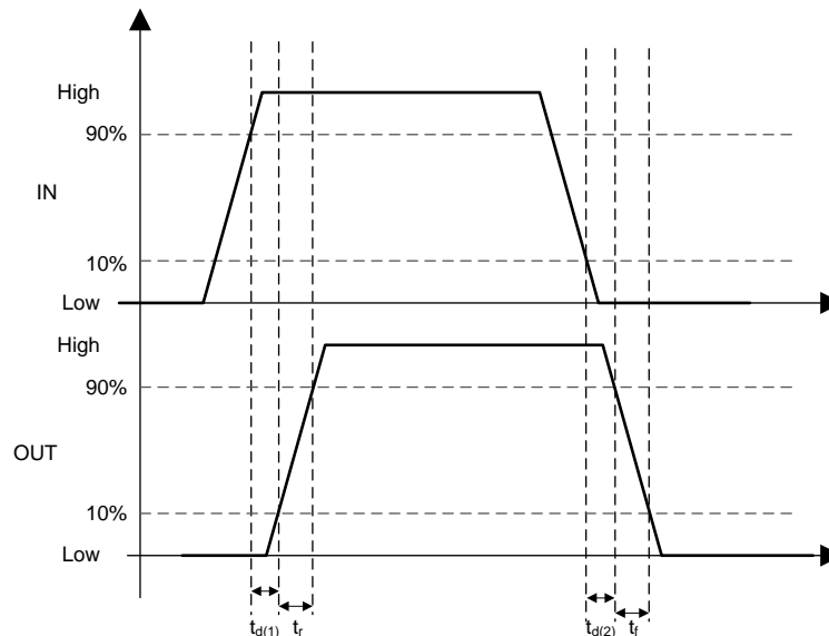
Figure 1. Input Driver Operation
