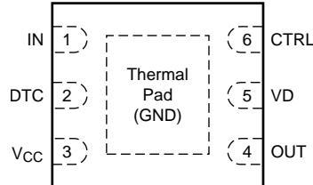
Pin Functions
