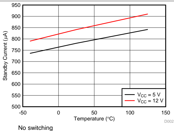
Figure 3. Standby Current ( I_{CC(ON)} ) vs Temperature
