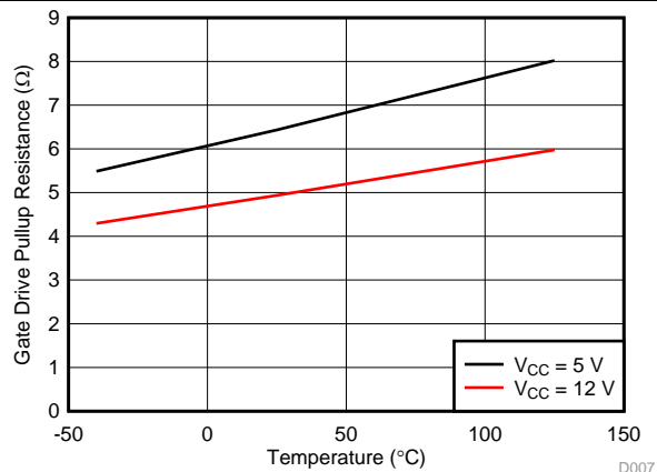
Figure 8. Gate-Drive Pullup Resistance ( R_{UP} ) vs Temperature
