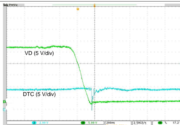
Figure 41. SR Turnon Edge After Optimization
