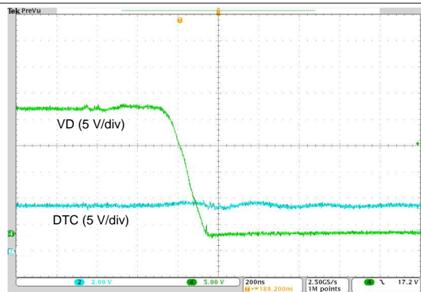
Figure 40. SR Turnon Edge Before Optimization
