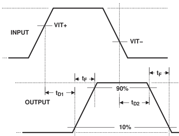
Figure 8-1. Timing Diagram
