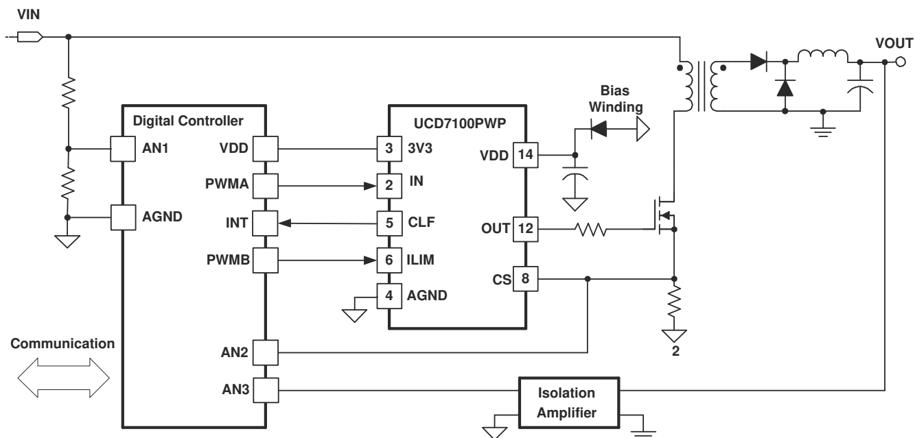
Figure 10-1. Typical Application
