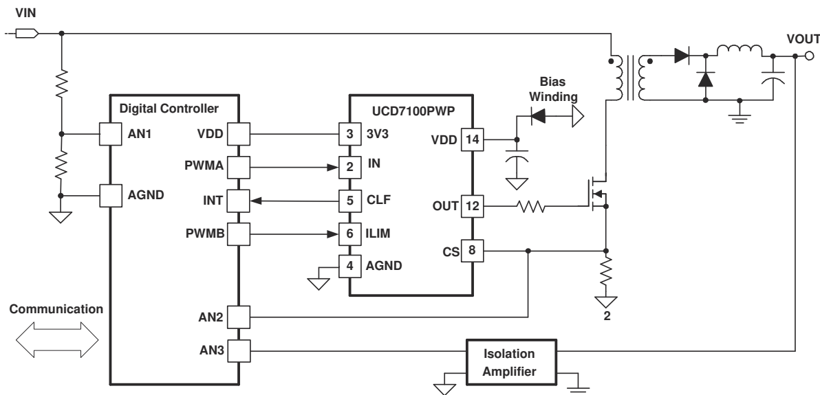
Simplified Schematic
