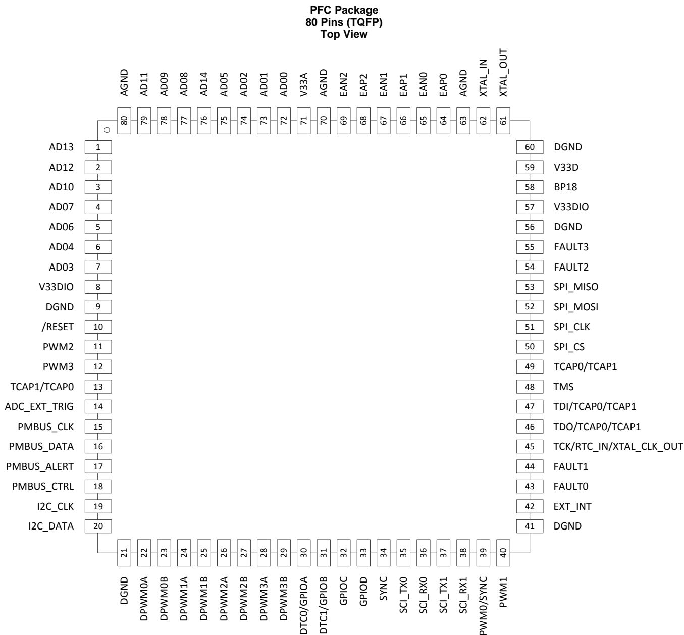
Pin Functions
