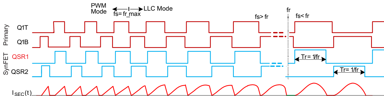
Figure 13. LLC Waveforms
