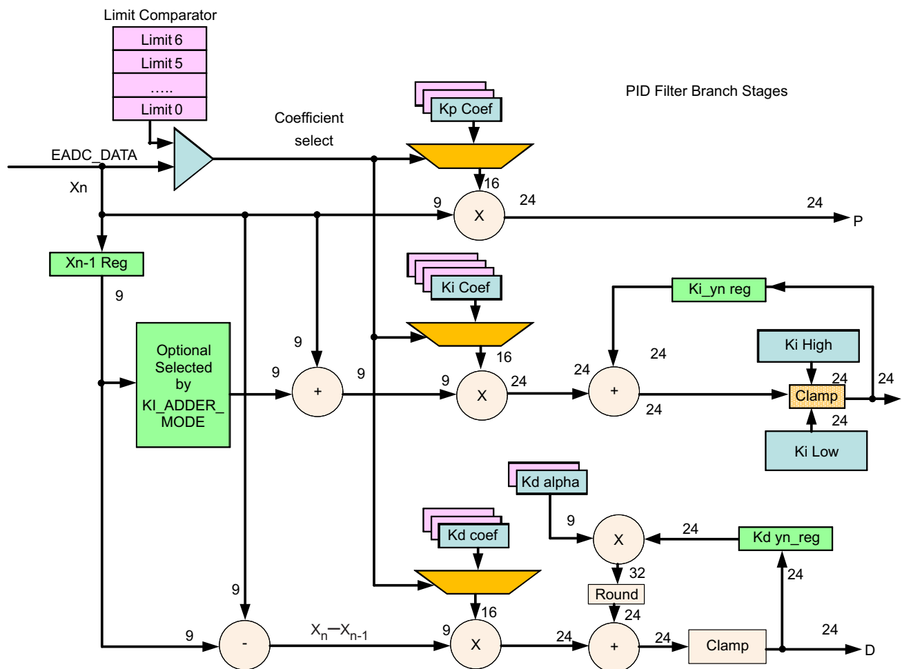
Figure 6-14. First Section of the Filter
