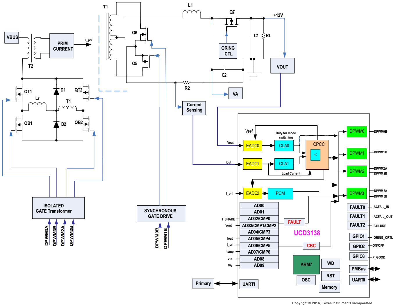
Figure 7-1. Phase-Shifted Full-Bridge
