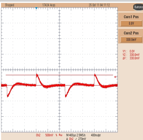
Figure 7-10. Load Transient
