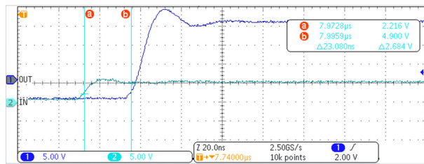
Figure 7-3. UCC5713x Rising (Turn-On) Propagation Delay
