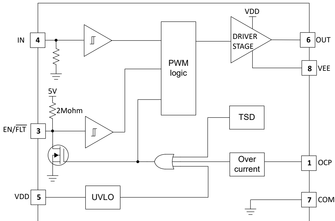
Figure 6-1. UCC5713xB Simplified Functional Block Diagram
