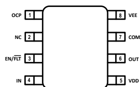
Figure 4-1. UCC5713xB 8-Pin SOIC D Package Top View
