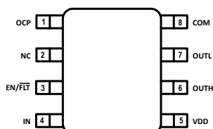
Figure 4-2. UCC5713xC SOIC D Package Top View
