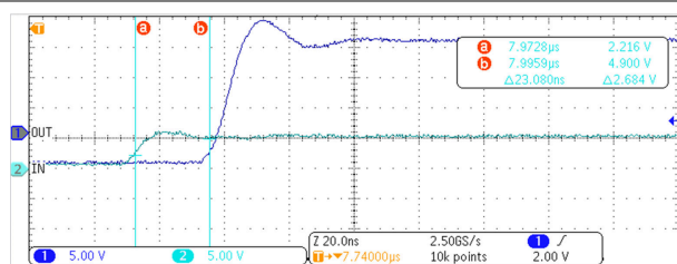
Figure 7-3. UCC57102Z-Q1 Rising (Turn-On) Propagation Delay
