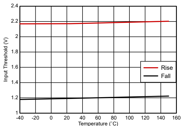
Figure 5-10. Input Threshold
