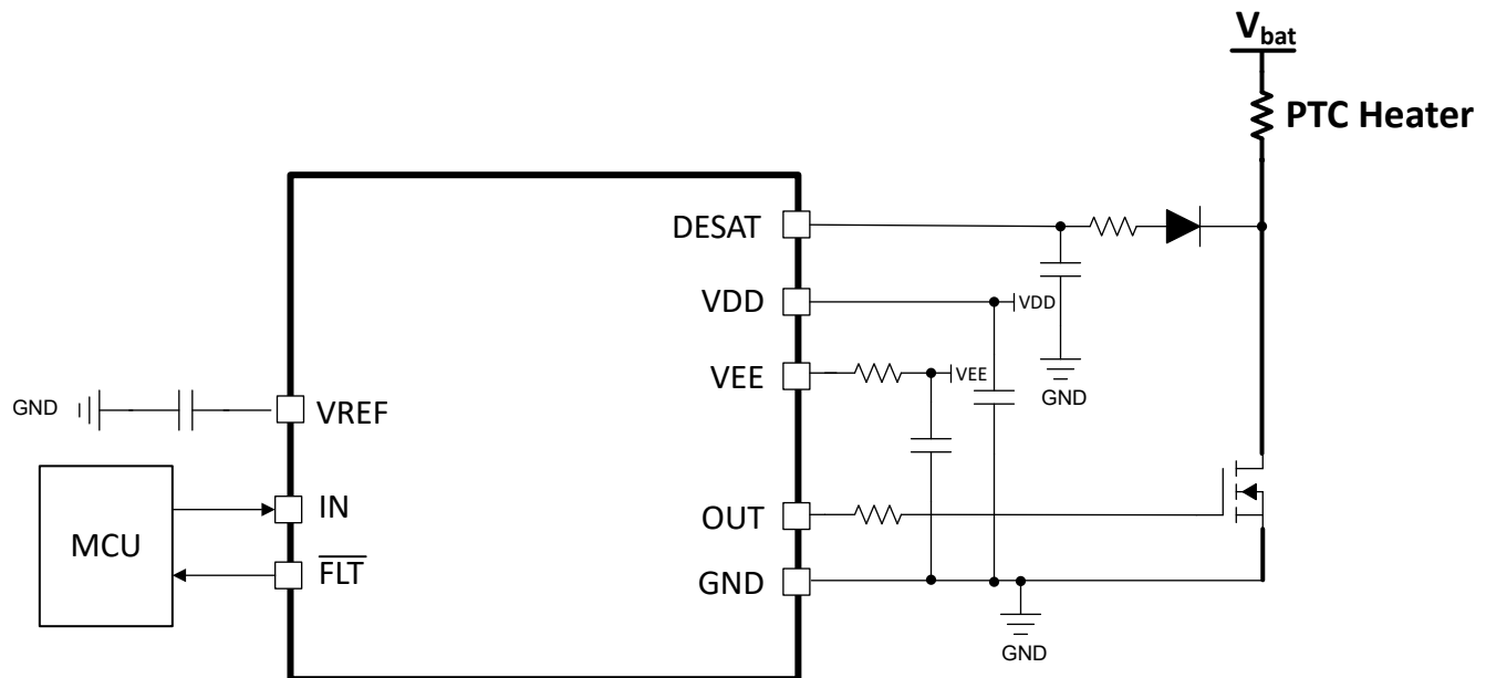
Figure 7-1. UCC57102Z-Q1 Used in a PTC Heater Application
