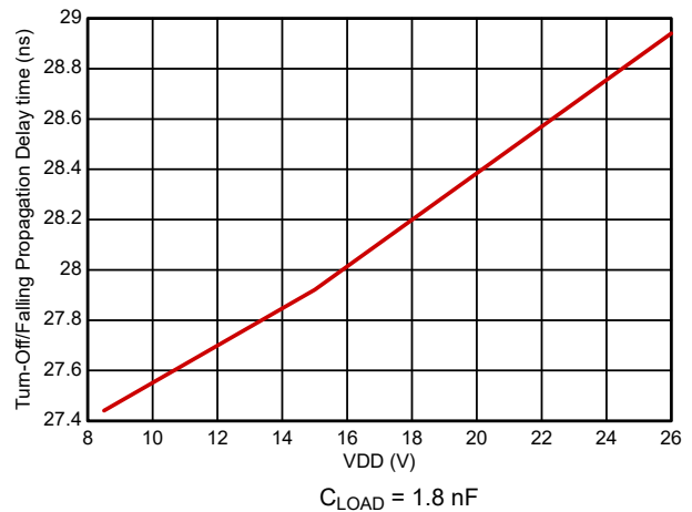
Figure 5-20. Input to Output Falling (Turnoff) Propagation Delay
