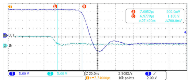
Figure 7-4. UCC57108 Falling (Turn-Off) Propagation Delay
