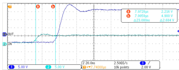
Figure 7-3. UCC57108 Rising (Turn-On) Propagation Delay
