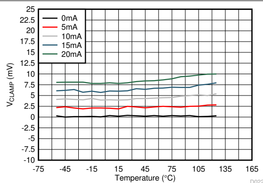
Figure 5-21. V_{CLAMP} vs Temperature
