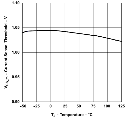
Figure 6-18. Current Sense Threshold Voltage vs Temperature
