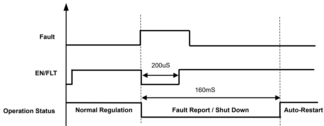
Figure 7-6. Auto-restart operation
