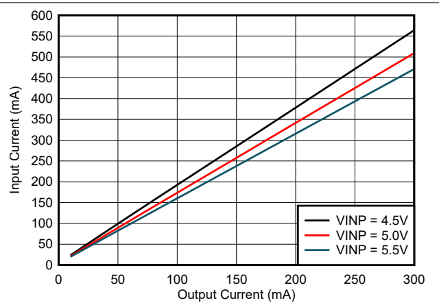
Figure 6-8. Input Current ( I_{VINP} ) vs Load Current ( I_{VCC} ): V_{CC} = 5.0V , T_A = 25^\circ C , C_{OUT2} = 22\mu F
