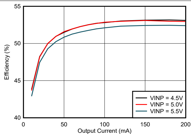
Figure 6-11. Efficiency vs Load Current (I VCC ): VCC = 5.5V, T A = 25°C, C OUT2 = 22μF
