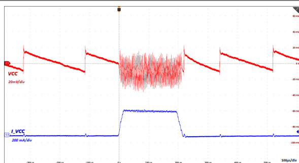
Figure 8-4. Load Transient: VINP = 5.0V, VCC = 5.0V , C OUT2 = 22µF , I VCC = 0mA - 300mA - 0mA
