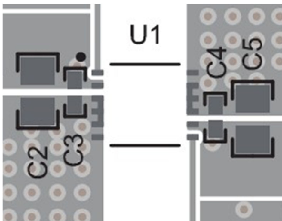
Figure 10-1. Layout Example
