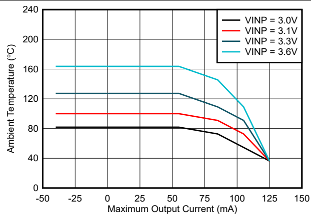
Figure 6-8. Maximum Output Current vs Ambient Temperature : VCC = 5.5V, C OUT2 = 22μF
