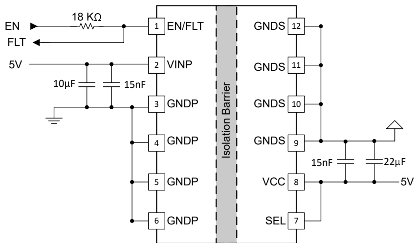
Figure 8-1. Typical Application
