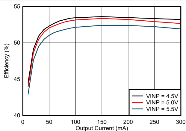
Figure 6-9. Efficiency vs Load Current (I VCC ): VCC = 5.0V, T A = 25°C, C OUT2 = 22μF
