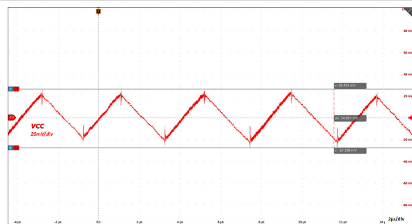
Figure 8-3. Steady State Output Voltage Ripple: VINP = 5.0V, VCC = 5.0V , C OUT2 = 22µF, 300mA Load
