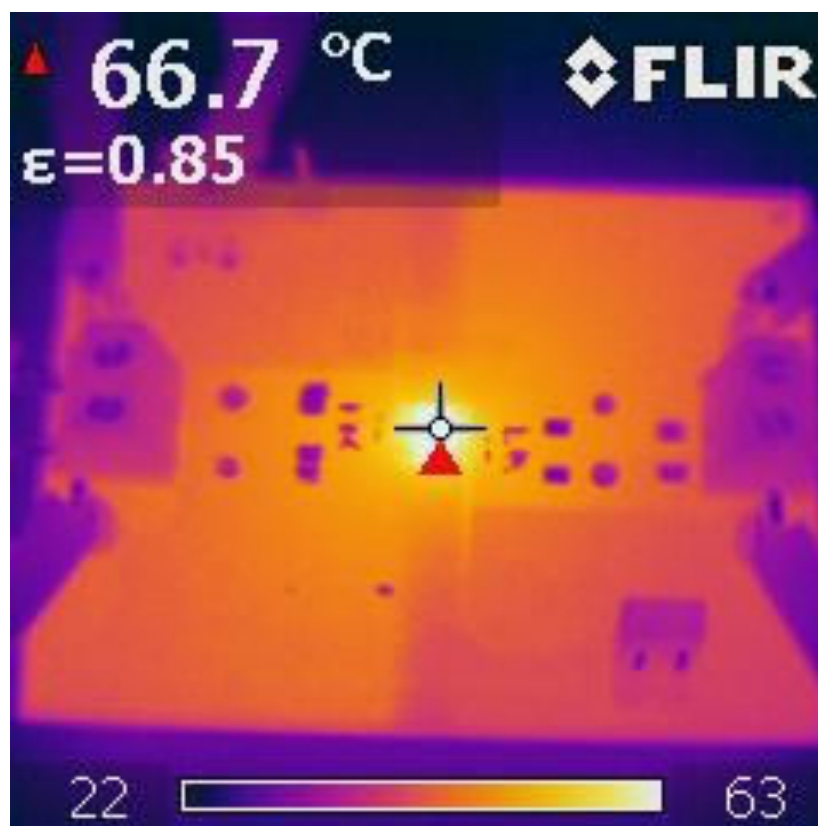
Figure 10-2. UCC33020 Thermal Image: VINP = 5.0V, VCC = 5.0V, P Out =1.0W
