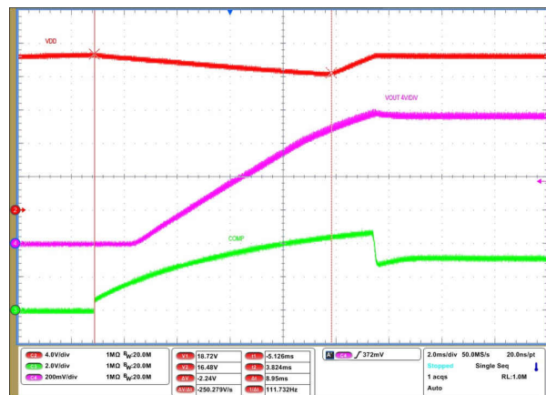
V DD capacitor hold-up time = 8.9 ms V OUT rise time = 9.1 ms CH2: VDD at 4 V/DIV CH3: COMP at 2V/DIV CH4: VOUT at 4 V/DIV via differential probe Figure 9-13. V OUT Soft Starting at 800 V IN , 40 W
