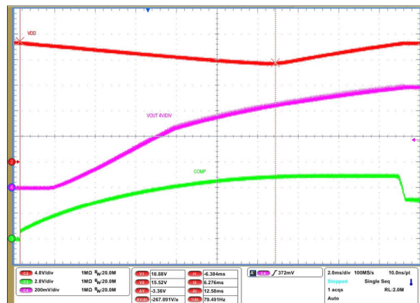
V DD capacitor hold-up time = 12.6 ms V OUT rise time = 17.2 ms CH2: VDD at 4 V/DIV CH3: COMP at 2V/DIV CH4: VOUT at 4 V/DIV via differential probe Figure 9-12. V OUT Soft Starting at 50 V IN , 20 W
