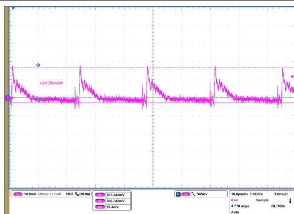
Output Voltage Ripple = 388 mV pp CH4: V_{OUT} at 200 mV/DIV via differential probe
