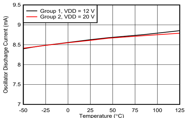
Figure 7-2. Oscillator Discharge Current vs Temperature
