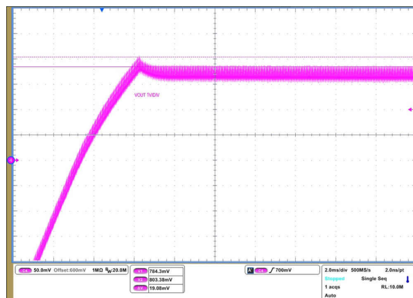
Soft Start Overshoot = 2.4 % CH4: V_{OUT} at 1 V/DIV via differential probe
