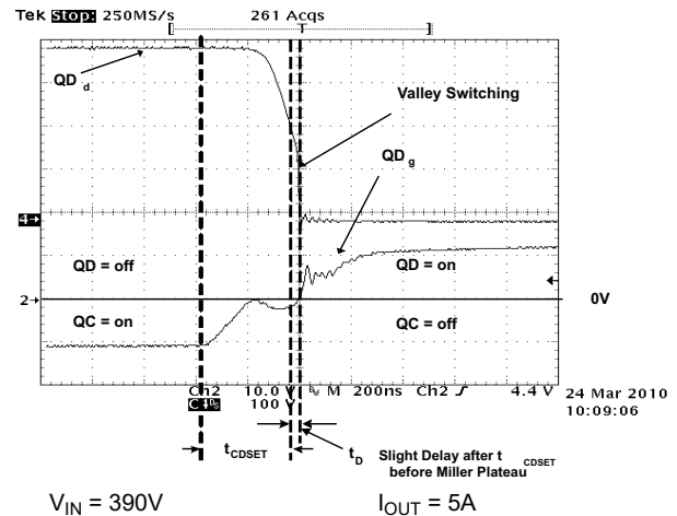
Figure 7-12. Full-Bridge Gate Drives and Primary Switch Nodes ( QD_g and QD_d )
