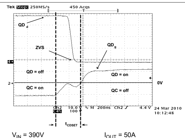
Figure 7-18. Full-Bridge Gate Drives and Switch Nodes (QD g QD d ) ZVS maintained from 50% to 100% output power
