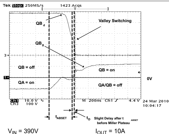
Figure 7-13. Full-Bridge Gate Drives and Switch Nodes ( QB_g and QB_d )
