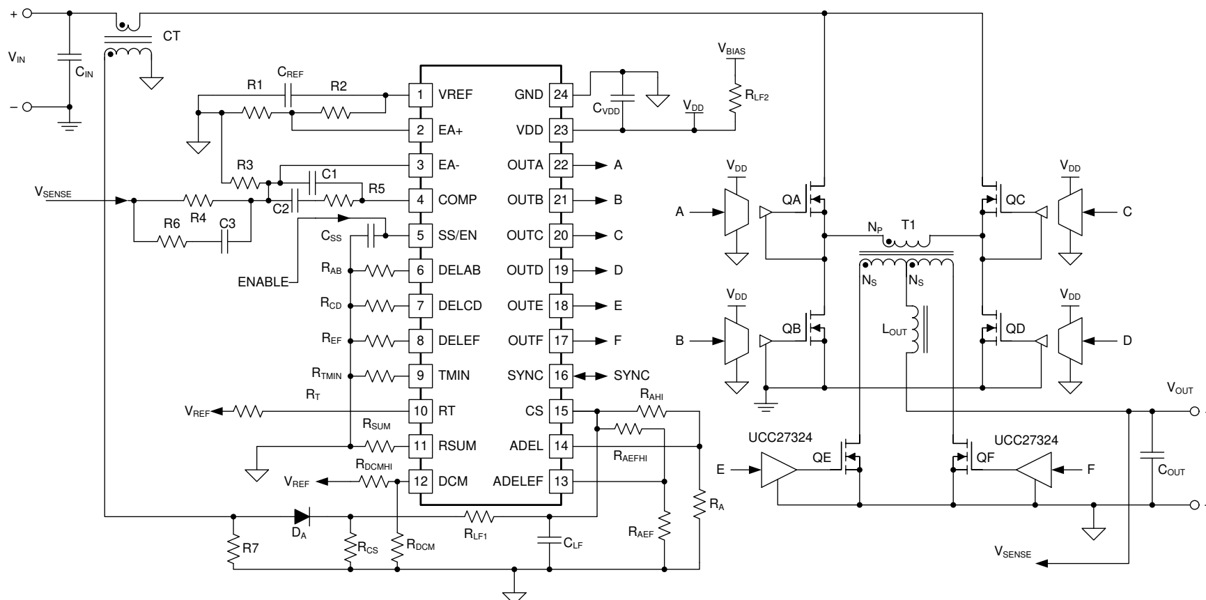
Figure 7-3. Typical Application
