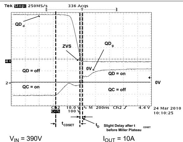
Figure 7-14. Full-Bridge Gate Drives and Switch Nodes ( QD_g and QD_d )
