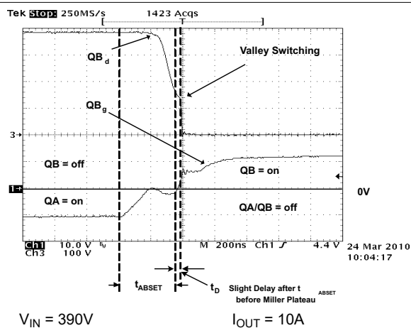
Figure 7-13. Full-Bridge Gate Drives and Switch Nodes (QB q QB d )
