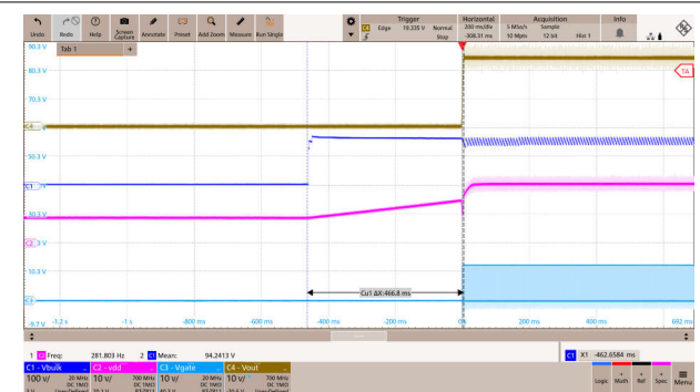
Figure 8-7. Start-Up Waveforms at 115Vac and Full Load
